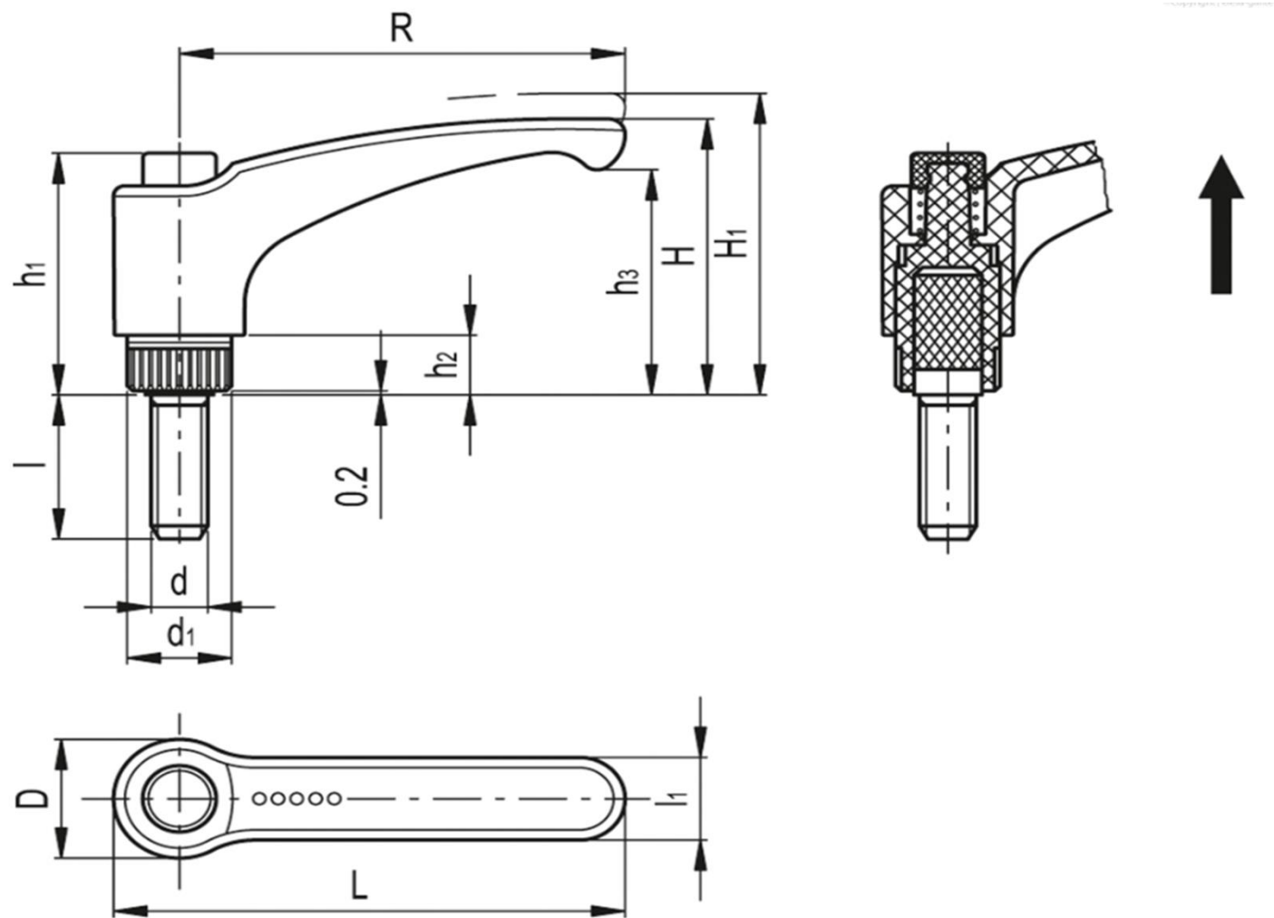
ERX.63 p-M8 x 40
