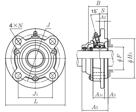
Cast dust cover type (Open end) C-UCFC...D1
