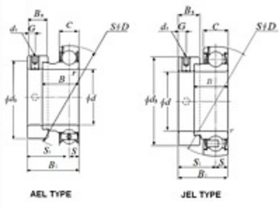
Bearing Insert w/ Eccentric Locking Collar, Narrow Inner Ring - Spherical O.D. - Dimensions
