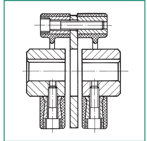
Double coupling, short series, elements arranged in series.
